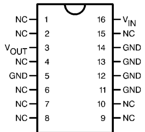
16-Lead Dual-in-Line Package (J)
